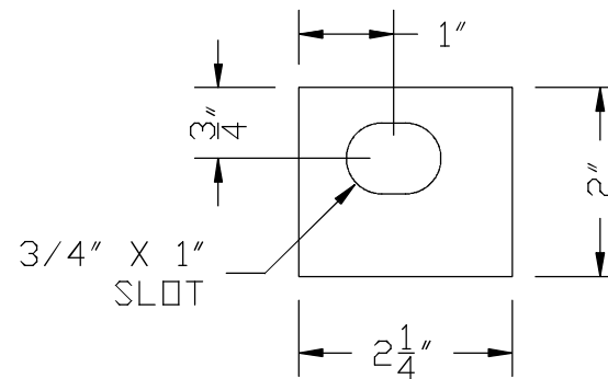
1/4" BOLT PAD DETAIL
